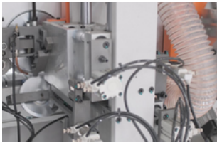
Flat scraping
